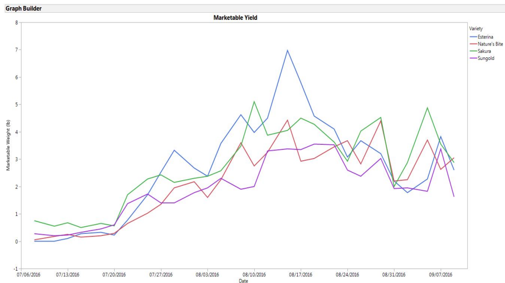
Figure 11. Variety yield over length of trial, Cherry Tomato Trials, Advancing Vegetable Production in NNY project, 2016. Key: • blue: Esterina • red: Nature's Bite • green: Sakura • purple Sungold.
