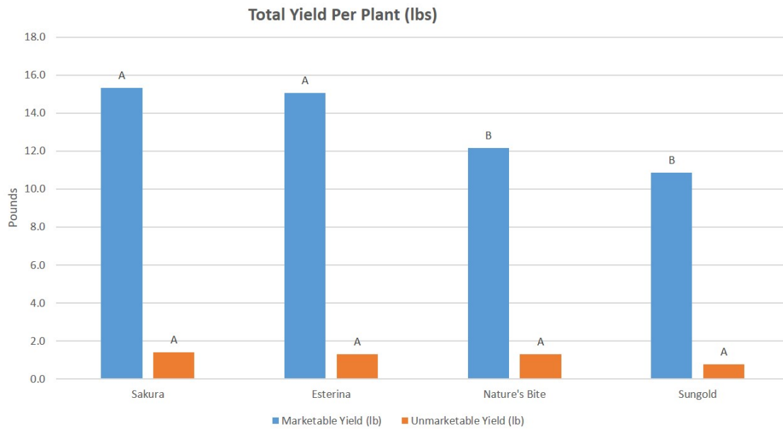
Figure 10. Total yield per plant in pounds, Cherry Tomato Trials, Advancing Vegetable Production in NNY project, 2016.
